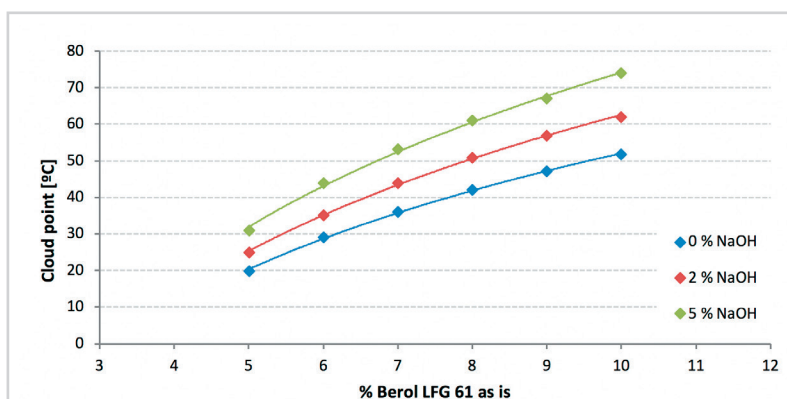
Fig. 4 Impact on cloud point of varying NaOH and Berol LFG 61 concentrations in a 10% GLDA chelating agent solution in demineralized water.
