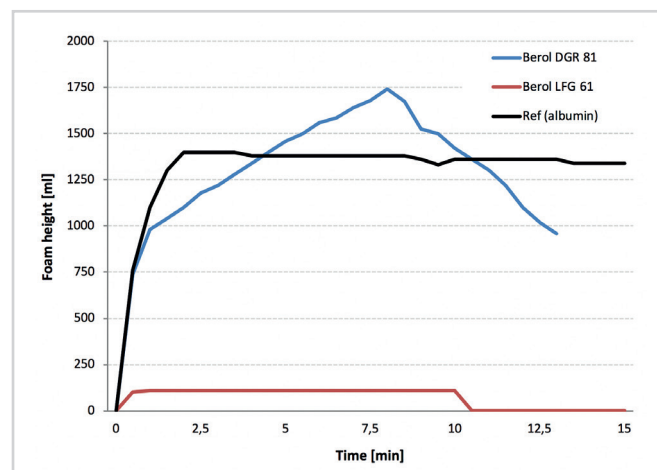
Fig. 1 Foaming profile for the different blends when tested in the circulation method (with circulation halted after 10 minutes). Albumin was used as foaming agent and the graph shows that Berol LFG 61 provides anti-foaming properties in this system, whilst Berol DGR 81 provides foaming.
